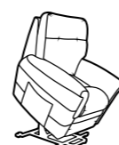
RISE & RECLINE Available in Power option H101cm W90cm D96cm SH51cm SD53cm SW47cm AH66cm Full Rise 137cm Full Recline 165cm
